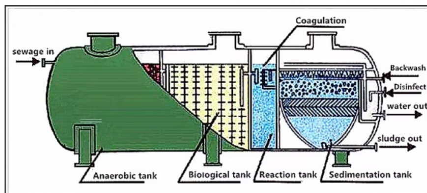
Sewage treatment processing of FRP storage tank
